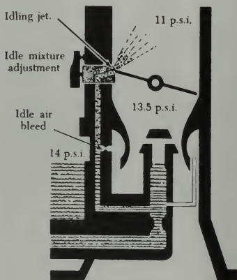
FIGURE 3-10. Idling system.
